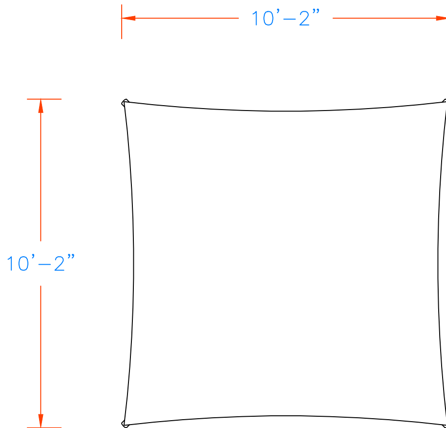
10' HYPERBOLIC UMBRELLA 10' x 10' (HYU101010SG) QRM503
