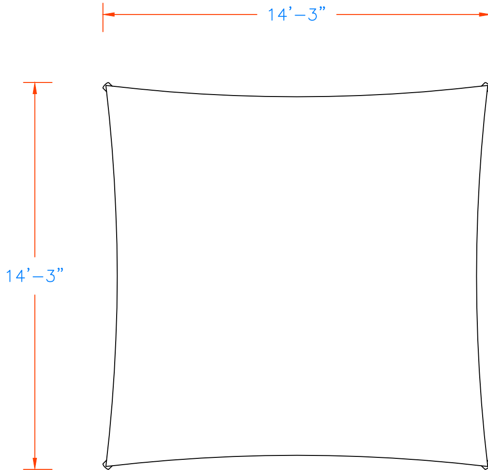
8' HYPERBOLIC UMBRELLA 14' x 14' (HYU141408SG) QRM499
