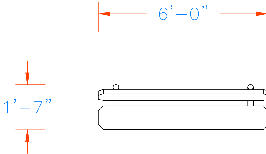
TUFFCLAD 6' BENCH w/BACK IN-GROUND (PS) 28009
